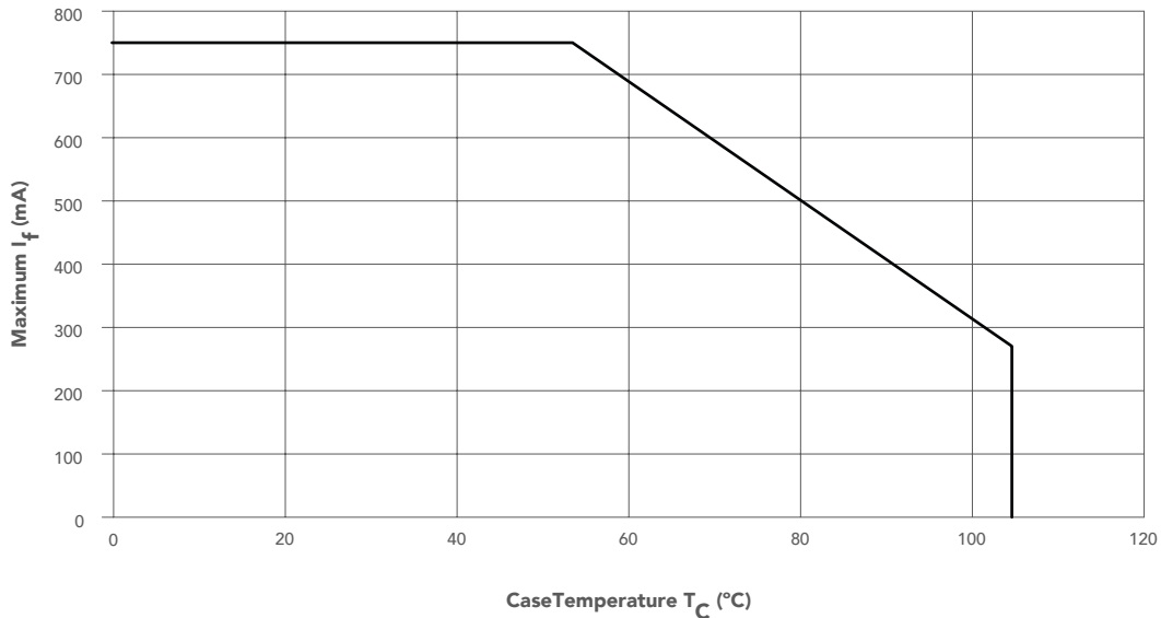
XOB09 Current Derating Curve
